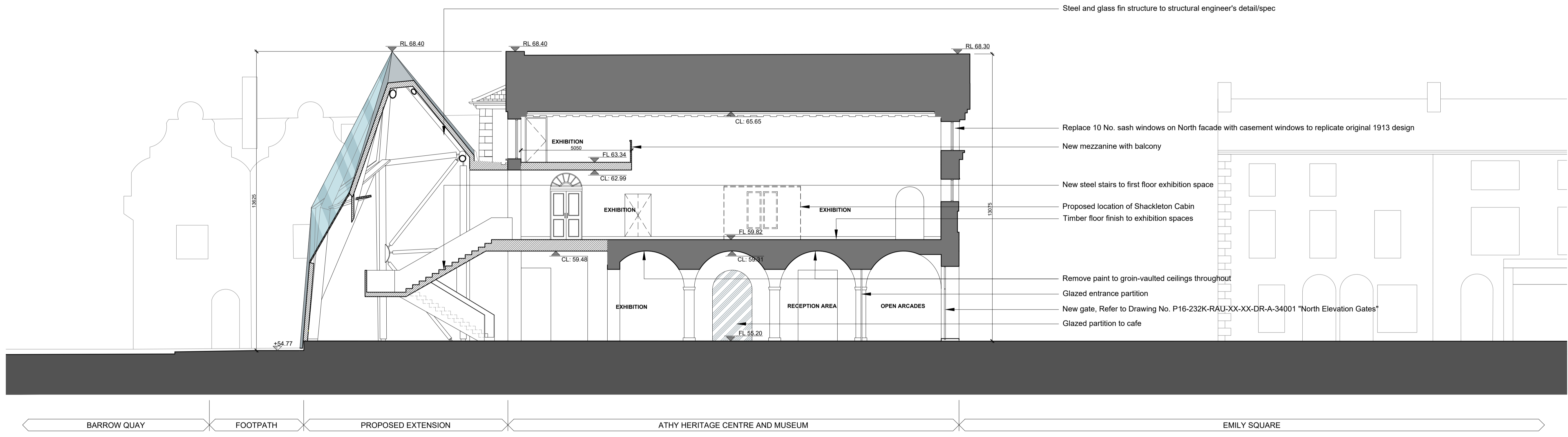
PROPOSED SECTION C-C 1:100@A1, 1:200@A3
